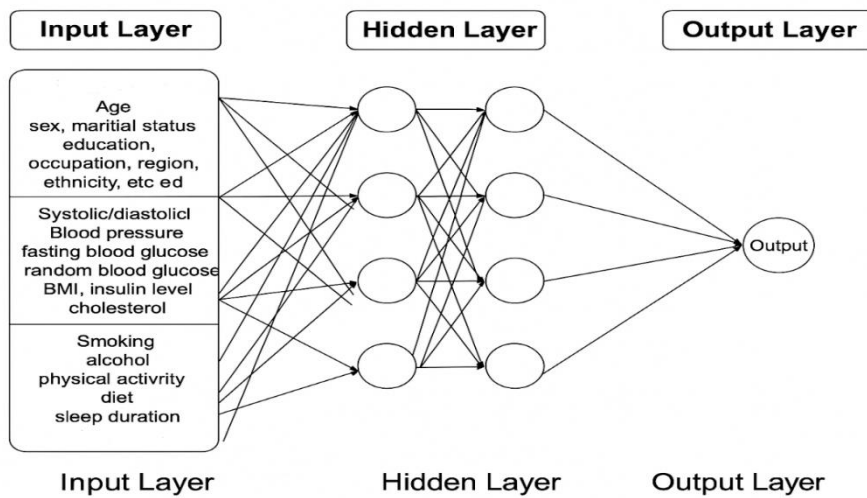
Figure 1: ANN Diagram
